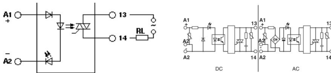
Circuit diagram
