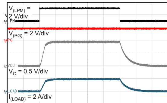
R_{(LOAD)} = 0.47\ \Omega Time = 50 \mu\text{s/div}
