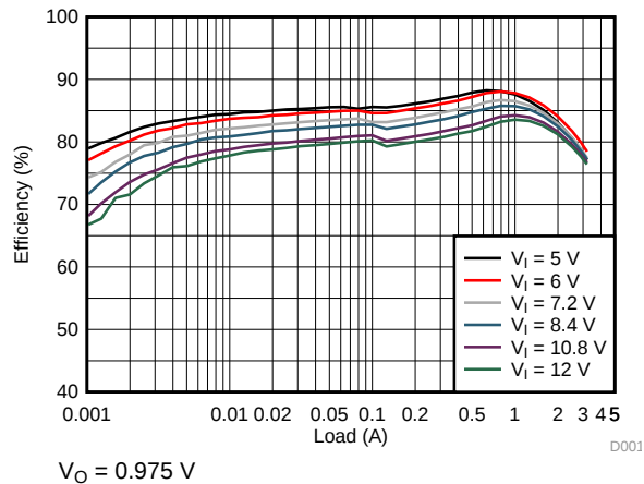
图 5. TPS62134A Efficiency
