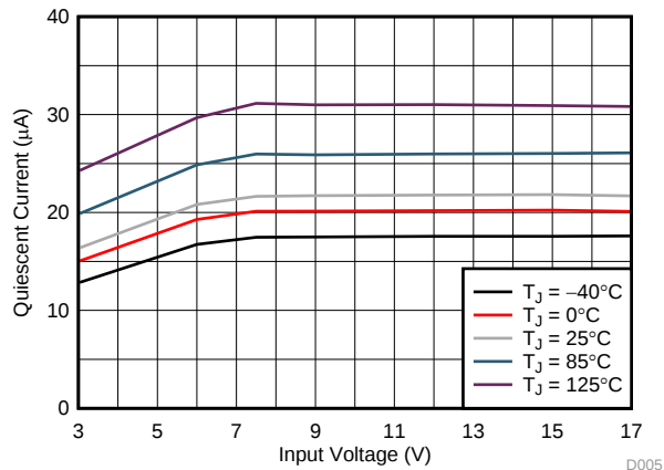
图 1. Quiescent Current into PVIN and AVIN
