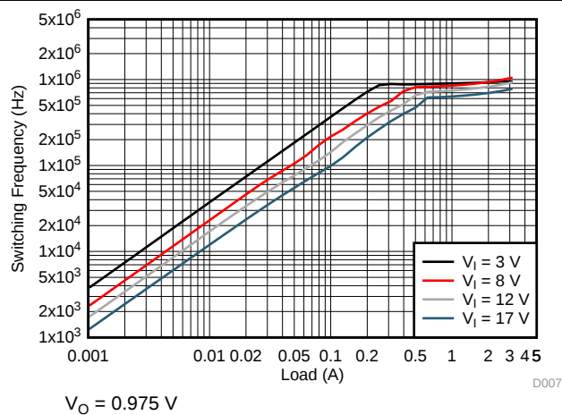
图 11. TPS62134A Switching Frequency
