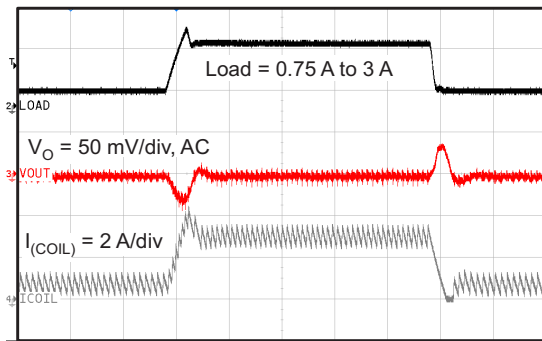
V_O = 0.95\text{ V} Time = 10 \mu\text{s/div}
