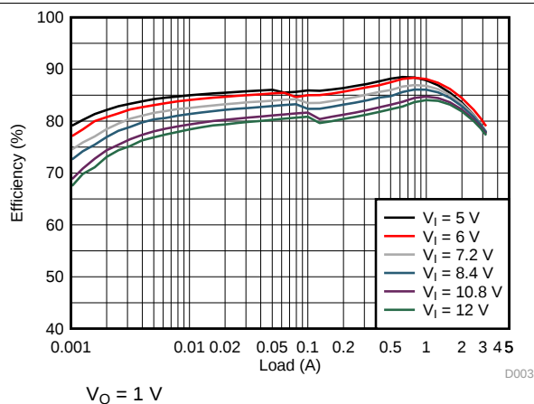
图 7. TPS62134C Efficiency
