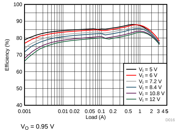
图 6. TPS62134B Efficiency
