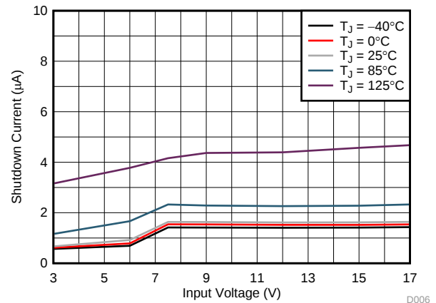
图 2. Shutdown Current into PVIN and AVIN
