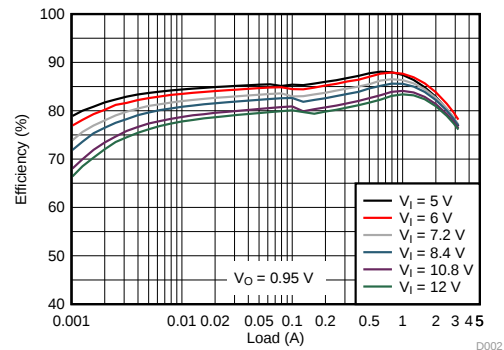
TPS62134A 效率
