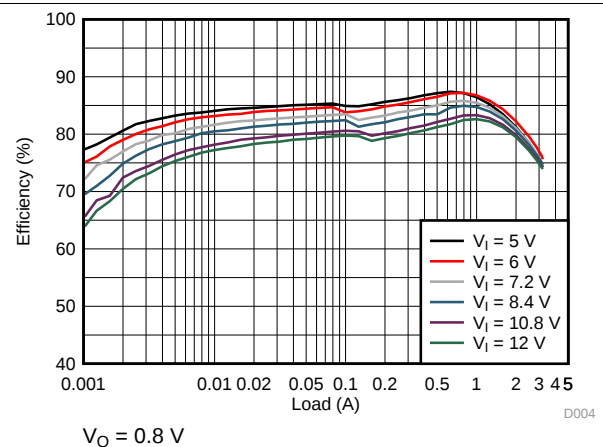
图 8. TPS62134C Efficiency
