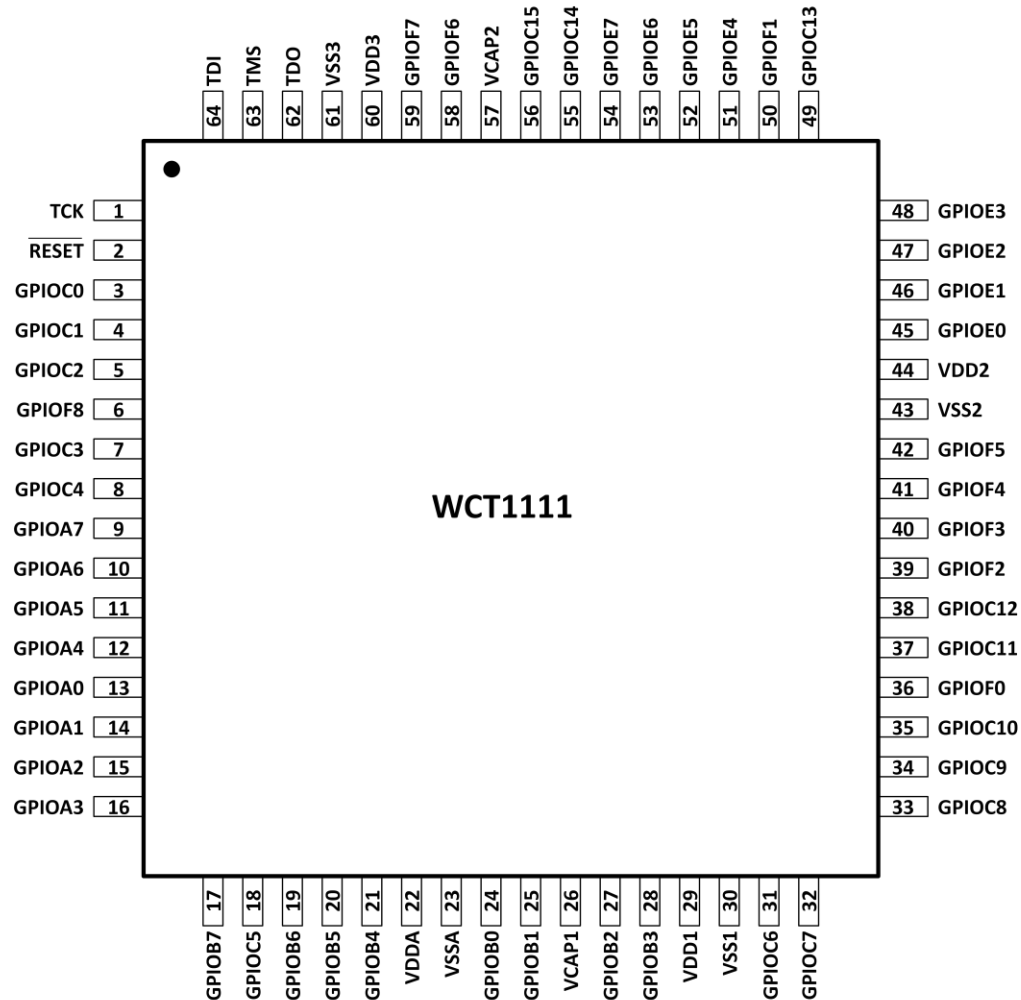
Figure 2. MWCT1111CLH pinout diagram
