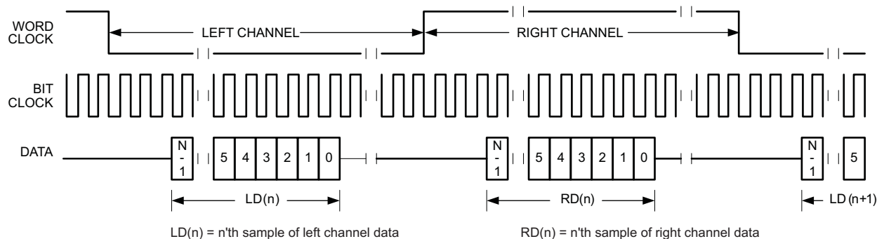
Figure 7-42. Timing Diagram for I²S Mode With Offset = 2
