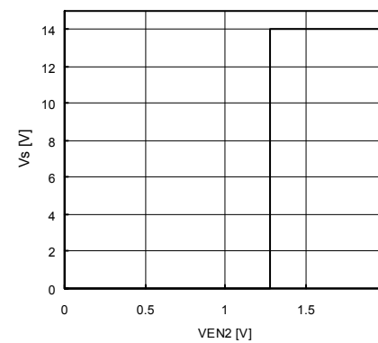
Fig.11 EN2 THRESHOLD VOLTAGE
