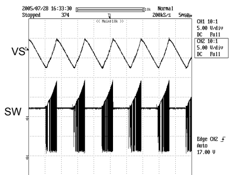
Fig.16 OVP WAVEFORM
