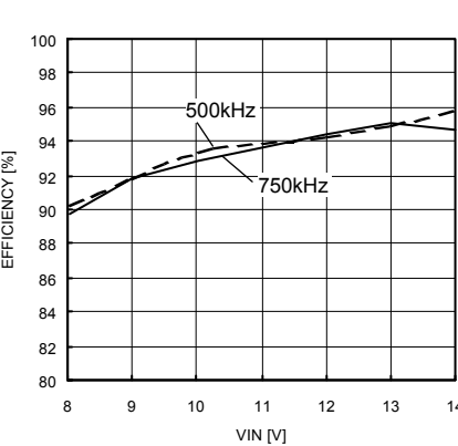
Fig.18 STEP UP EFFICIENCY
