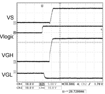
Fig.21 START UP WAVEFORM
