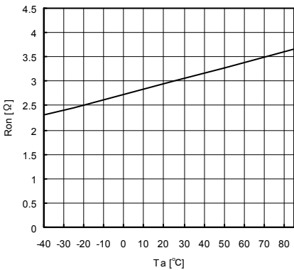
Fig.15 DRN ON RESISTANCE
