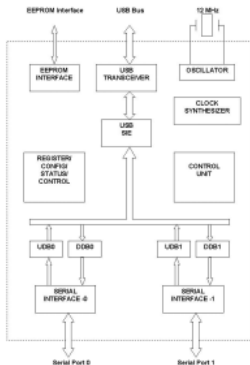
PL-2313 Block Diagram
