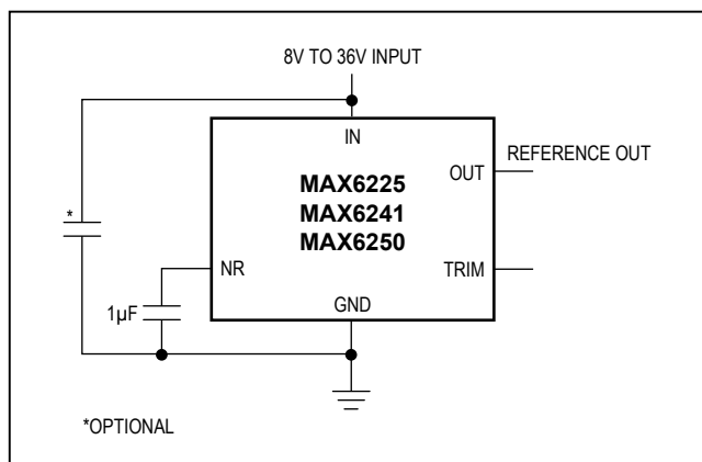
Figure 2. Noise-Reduction Capacitor
