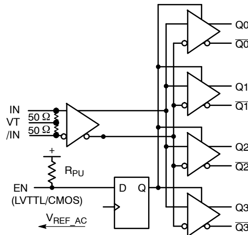
Figure 1. Logic Diagram
