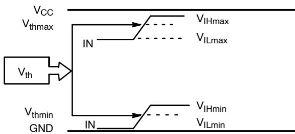
Figure 21. V_{th} Diagram
