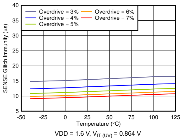
图 6-20. SENSE Glitch Immunity vs Temperature
