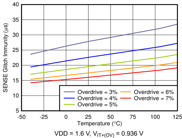
图 6-18. SENSE Glitch Immunity vs Temperature
