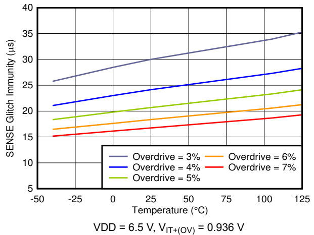
图 6-19. SENSE Glitch Immunity vs Temperature
