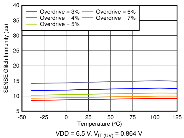
图 6-21. SENSE Glitch Immunity vs Temperature
