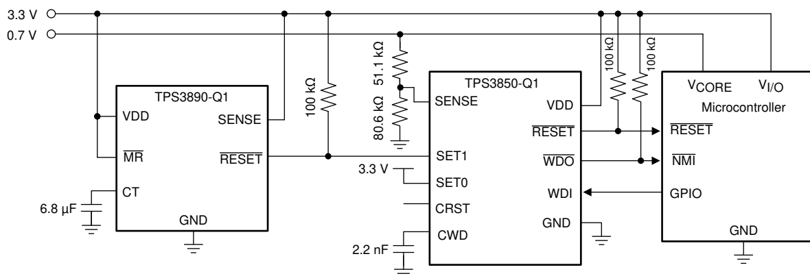
图 8-12. Monitoring Supply Voltage and Watchdog Supervision of a Microcontroller
