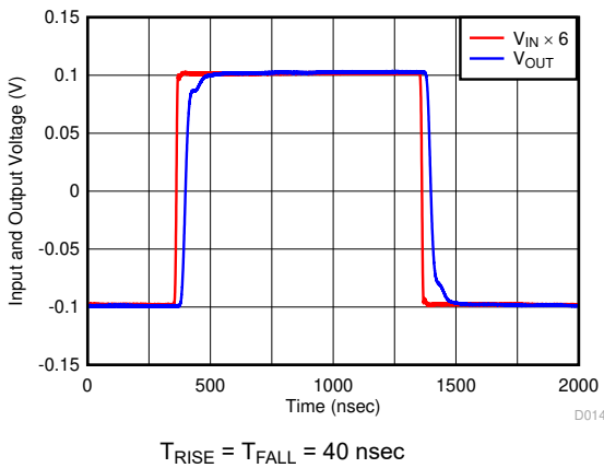
Figure 7-15. Small-Signal Transient Response
