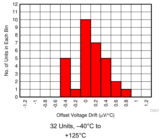
Figure 7-22. Input Offset Drift Distribution
