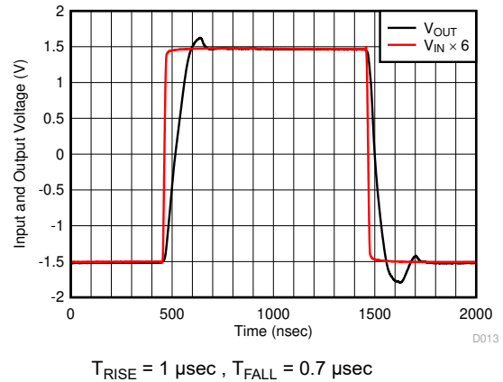
Figure 7-14. Large-Signal Transient Response
