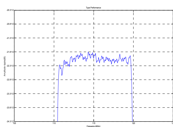
Passband Response
