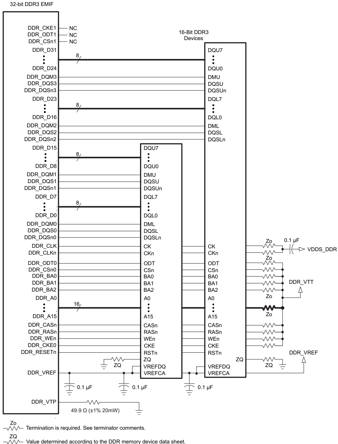
Figure 5-52. 32-Bit DDR3 Interface Using Two 16-Bit DDR3 Devices With V_{\Pi} Termination
