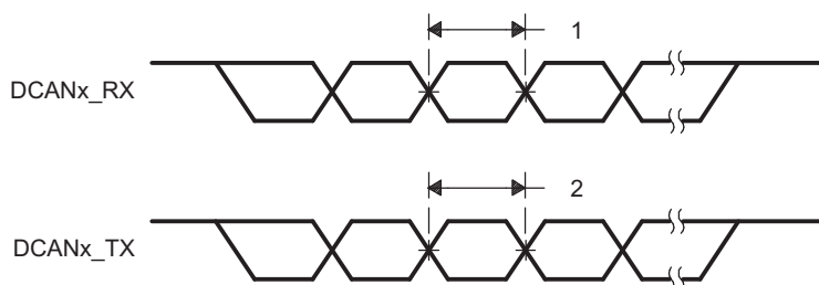
Figure 5-17. DCANx Timings
