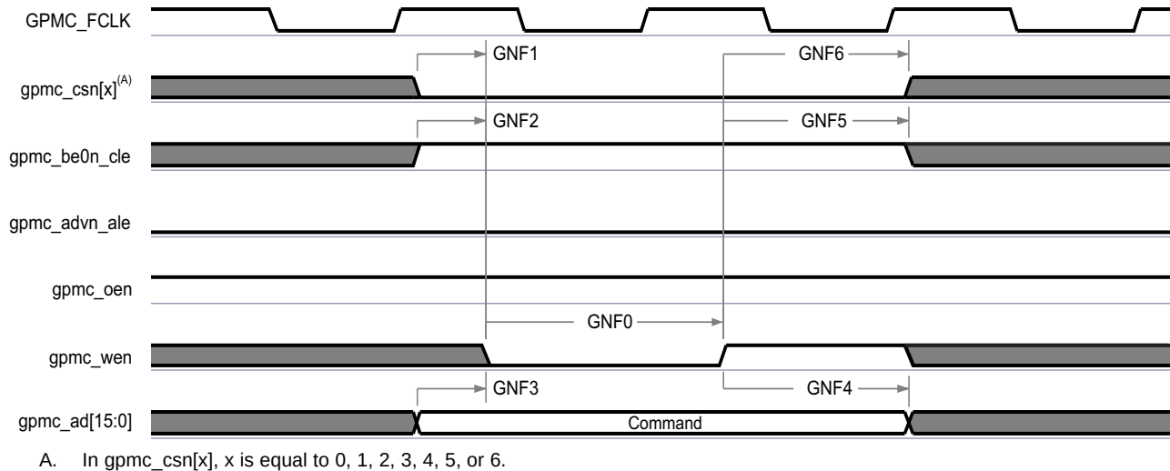
Figure 5-44. GPMC and NAND Flash—Command Latch Cycle
