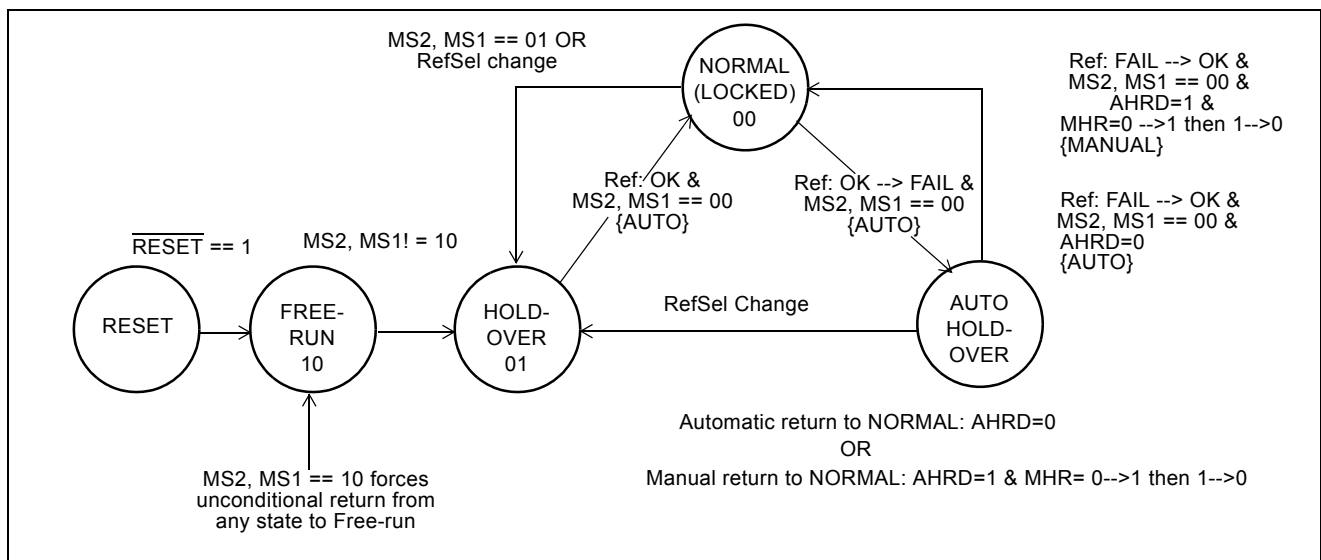
Figure 8 - Automatic Entry into Auto Holdover State and Eecoverly into Normal mode
