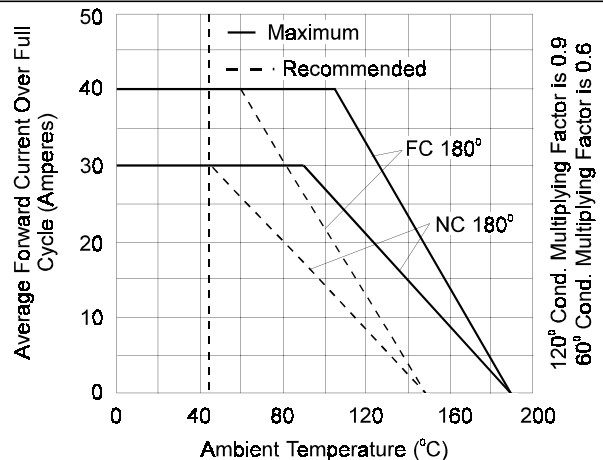
Fig. 6 - Diode Mounted on Heat Sink Type K3 with \theta_{HA} - NC 2.5^\circ\text{C/W} , FC 0.65^\circ\text{C/W}
