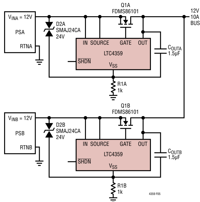
Figure 5. Redundant Power Supplies
