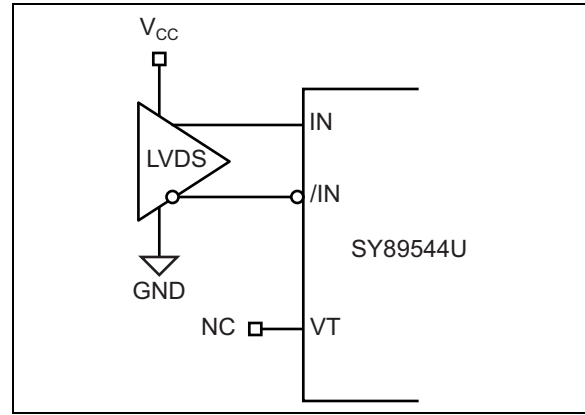
FIGURE 7-5: LVDS Interface.
