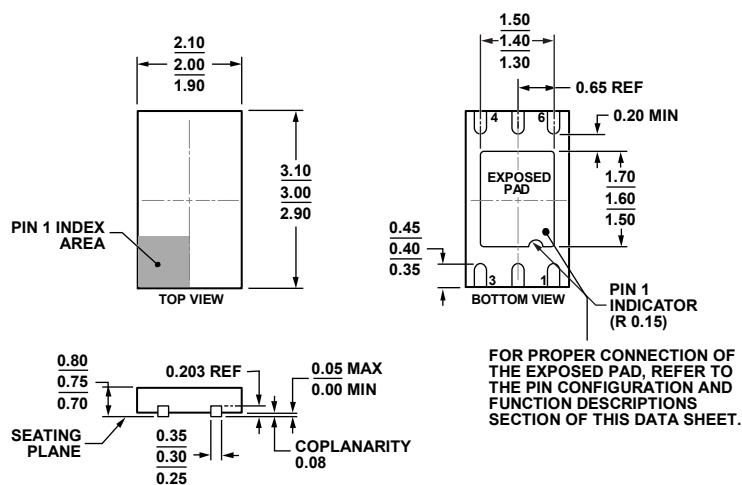
COMPLIANT TO JEDEC STANDARDS MO-229 Figure 55. 6-Lead Lead Frame Chip Scale Package [LF CSP_WD] 2.00 × 3.00 mm Body, Very Very Thin, Dual Lead (CP-6-5) Dimensions shown in millimeters
