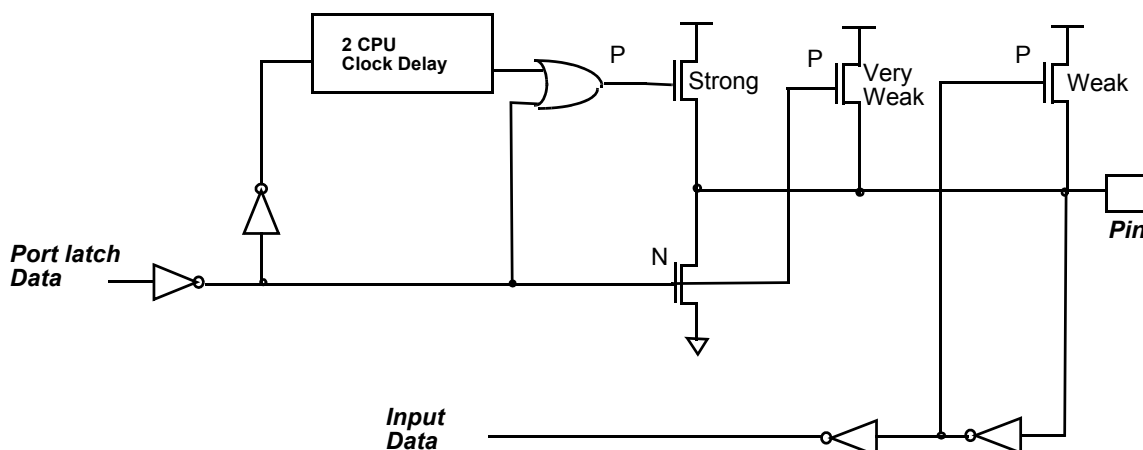
Figure 3. Quasi-Bi-directional Output
