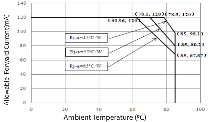
Ambient Temperature-Allowable Forward Current
