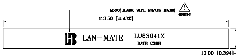
Label Drawing
