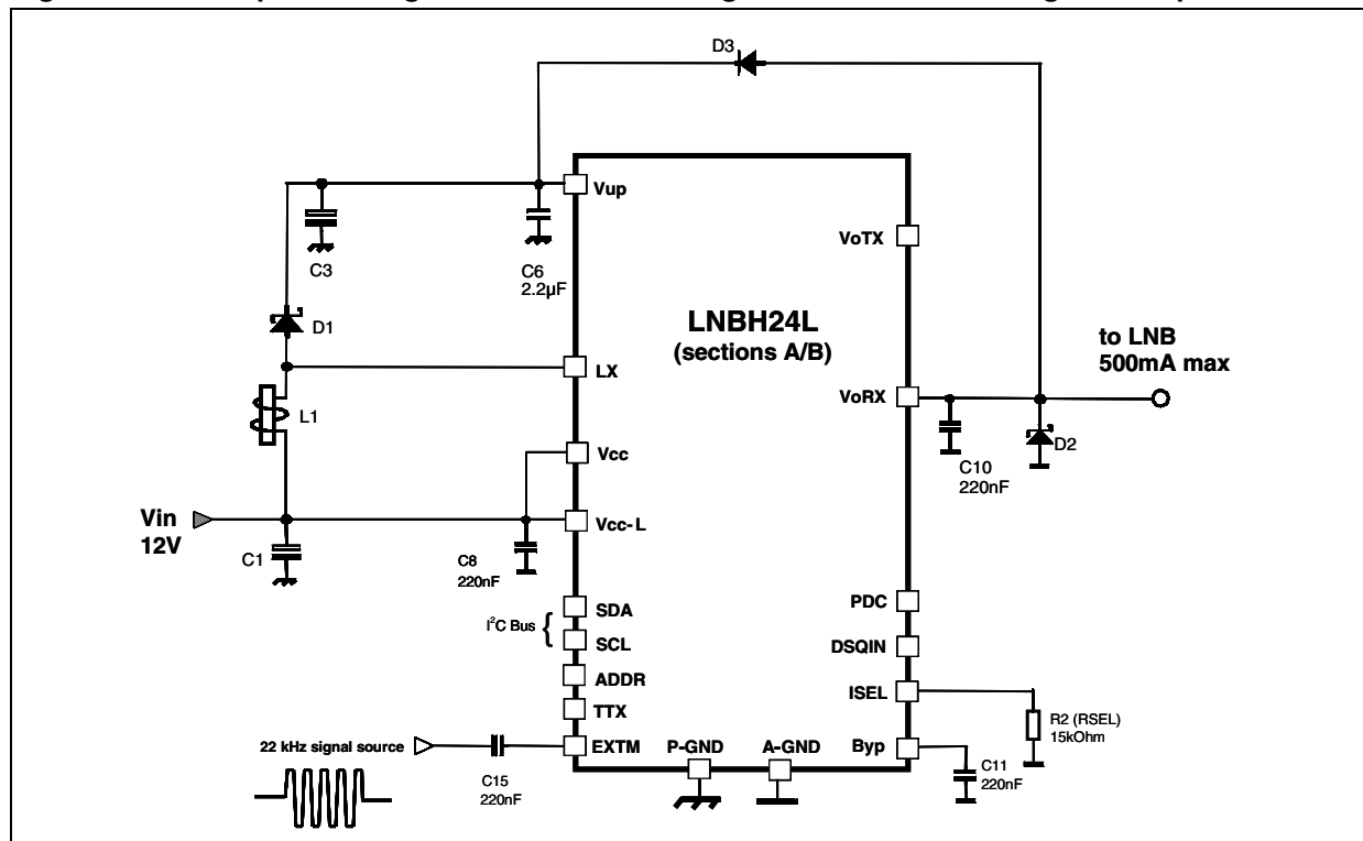
Figure 4. DiSEqC 1.x using external 22 kHz tone generator source through EXT pin
