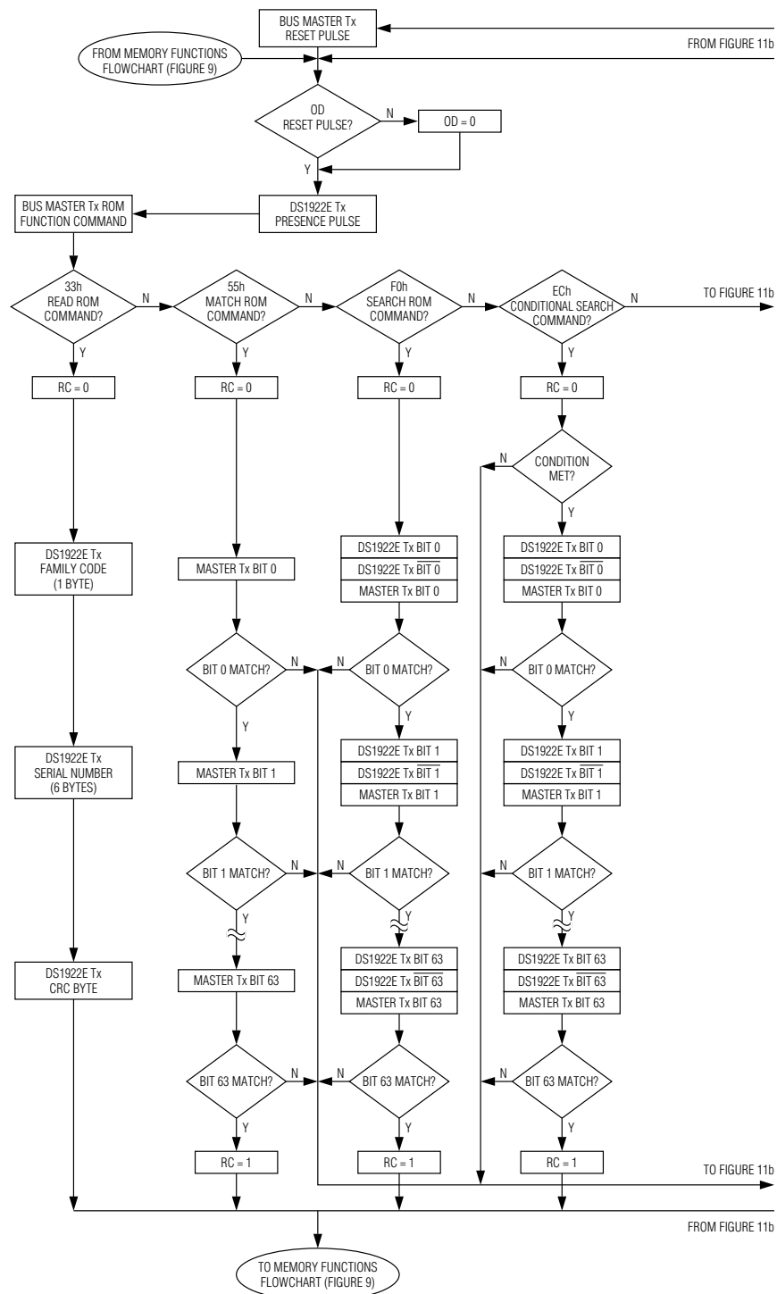
Figure 11a. ROM Functions Flowchart
