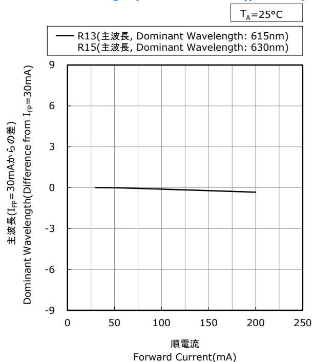
順電流-主波長( I_{FP}=30\text{mA} からの差)特性 Forward Current vs Dominant Wavelength (Difference from I_{FP}=30\text{mA} )
