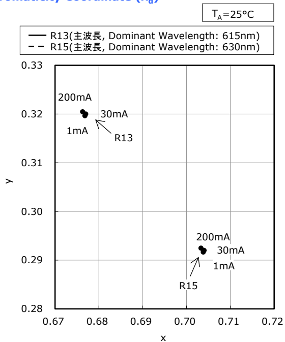
順電流-色度(主波長)特性 Forward Current vs Chromaticity Coordinate ( \lambda_d )
