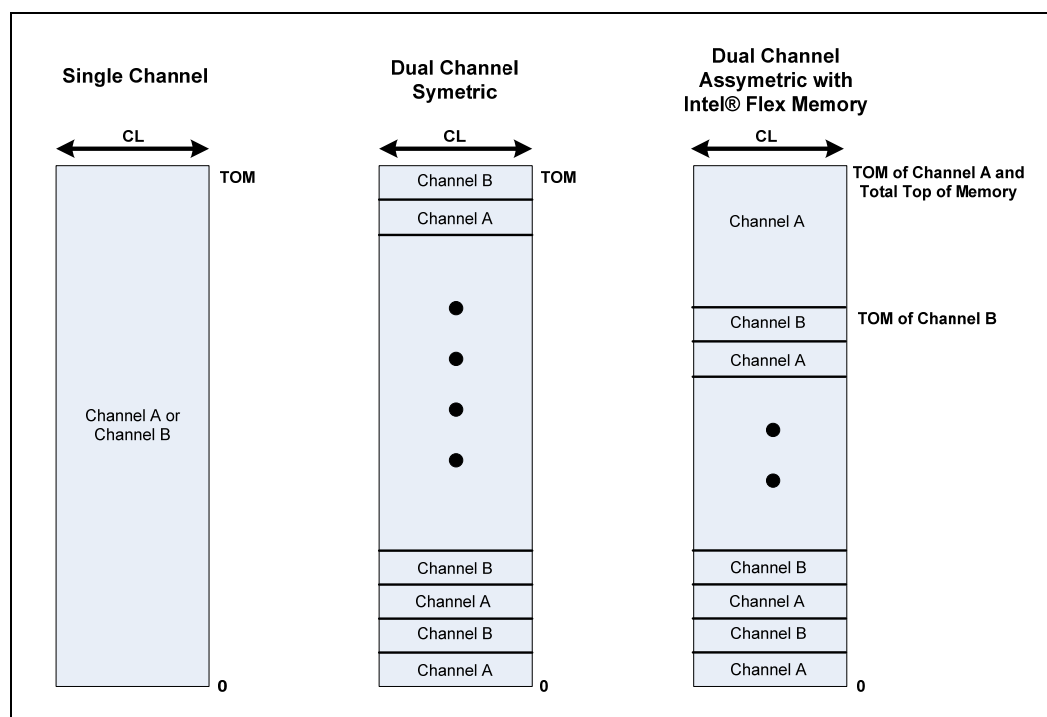
Figure 10-1. System Memory Styles
