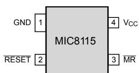
4-Lead SOT-143
