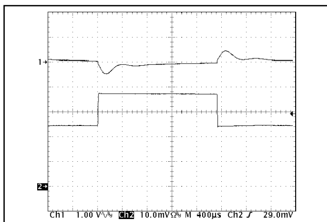
Figure 11: Output voltage response to step-change in load current (50%-75%-50% of I_{out(max)} ; dI/dt = 0.1A/\mu s ). Load cap: 200μF, 450 mΩ ESR electrolytic cap and 1μF ceramic cap. Top trace: V_{out} (1V/div), Bottom trace: I_{out} (1A/div).
