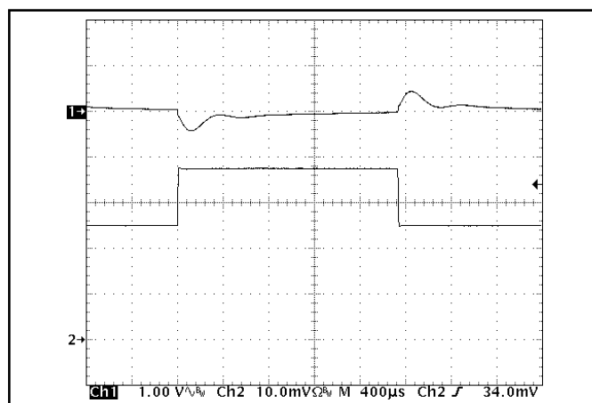
Figure 12: Output voltage response to step-change in load current (50%-75%-50% of I_{out(max)} ; dI/dt = 1A/\mu s ). Load cap: 200μF, 450 mΩ ESR electrolytic cap and 1μF ceramic cap. Top trace: V_{out} (1V/div), Bottom trace: I_{out} (1A/div).
