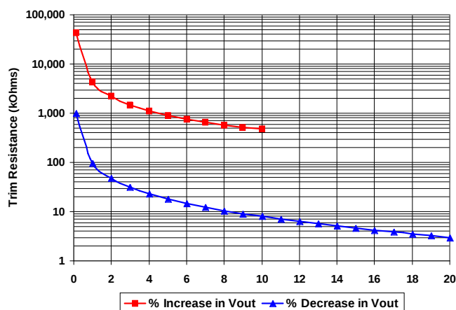
Figure C: Trim Graph for 54Vout module
