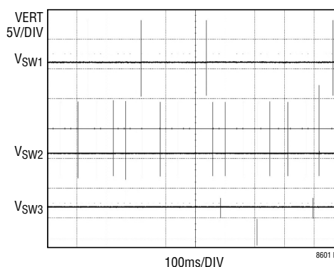
Figure 5. Burst Mode Operation SW Waveforms with All Channels in Burst Mode Operation
