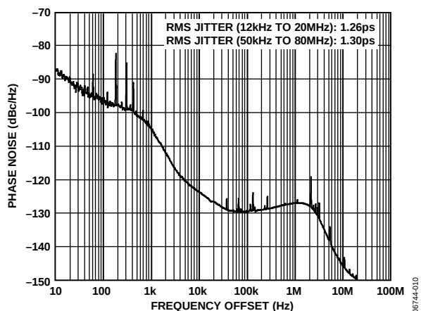
Figure 10. Additive Phase Noise at HSTL Output Driver, SYSCCLK = 1\text{ GHz} ( SYSCCLK\text{ PLL Enabled and Driven by a }25\text{ MHz Fox Crystal Oscillator} ), f_{REF} = 19.44\text{ MHz} , f_{OUT} = 155.52\text{ MHz} , DPLL\text{ Loop BW} = 1\text{ kHz}
