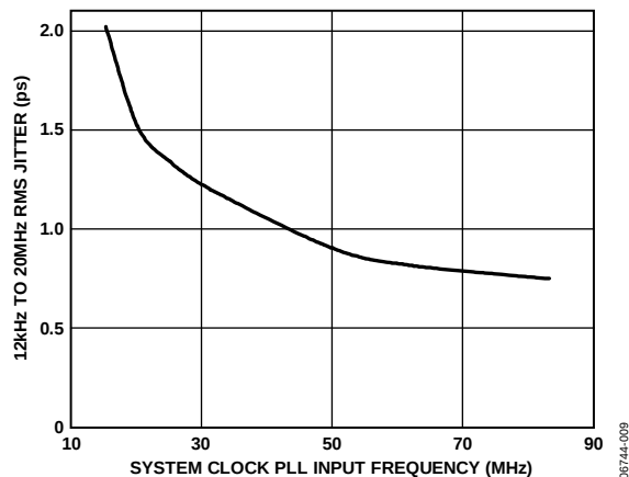
Figure 9. 12 kHz to 20 MHz RMS Jitter vs. System Clock PLL Input Frequency, SYSCCLK = 1\text{ GHz} , f_{REF} = 19.44\text{ MHz} , f_{OUT} = 155.52\text{ MHz}
