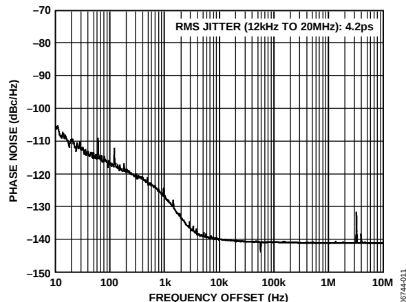
Figure 11. Additive Phase Noise at HSTL Output Driver, SYSCCLK = 500\text{ MHz} ( SYSCCLK\text{ PLL Disabled} ), f_{REF} = 10.24\text{ MHz} , f_{OUT} = 20.48\text{ MHz} , DPLL\text{ Loop BW} = 1\text{ kHz}
