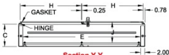
Section Y-Y
