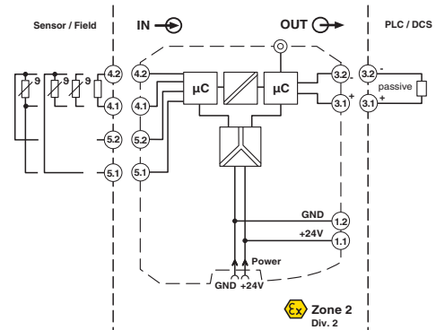
Block diagram
