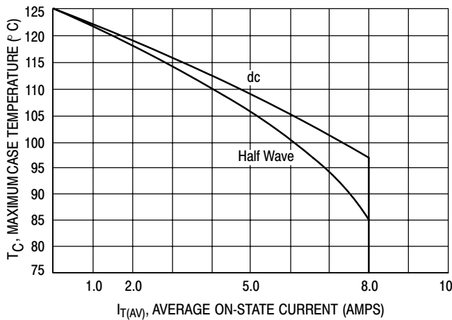
Figure 3. Current Derating
