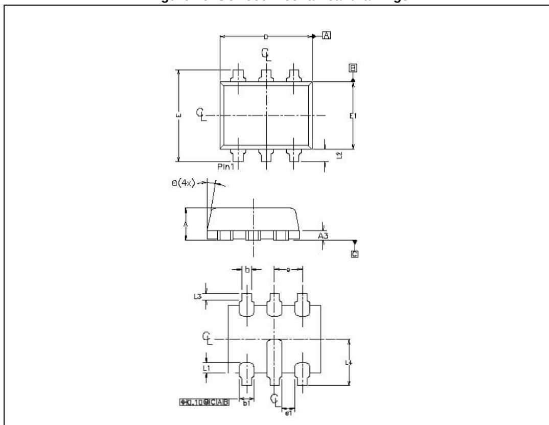
Figure 16. SOT666 mechanical drawings
