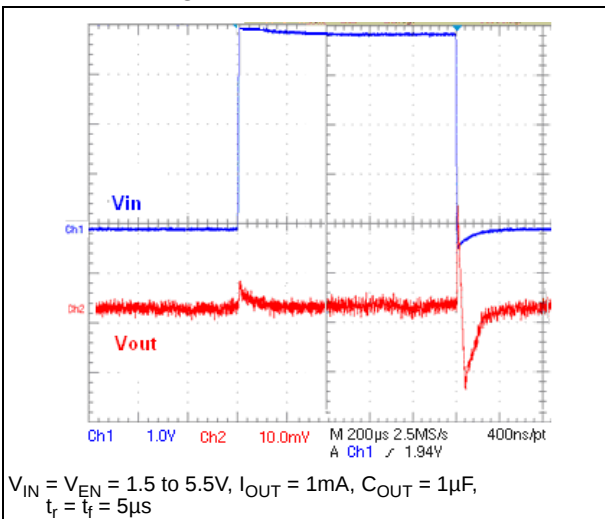
Figure 12. Line transient
