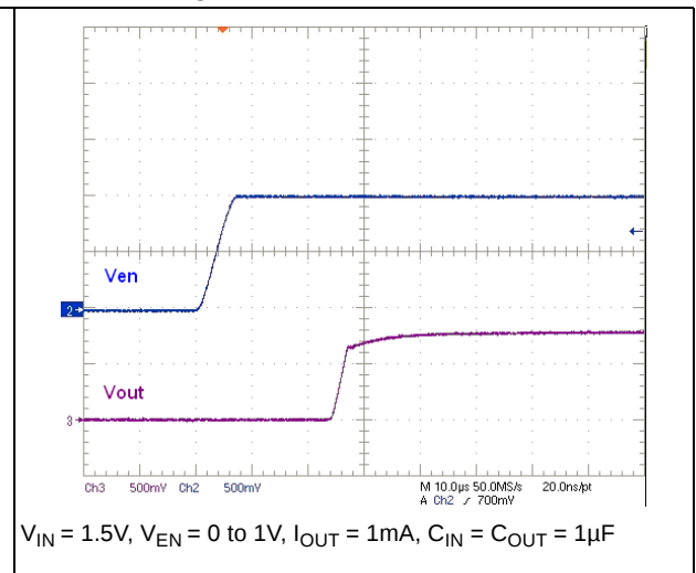
Figure 13. Enable transient
