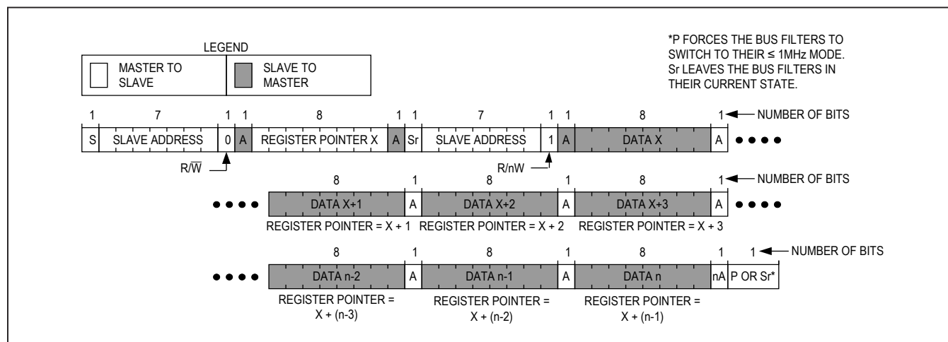
Figure 16. Reading Continuously from Sequential Registers X to N
