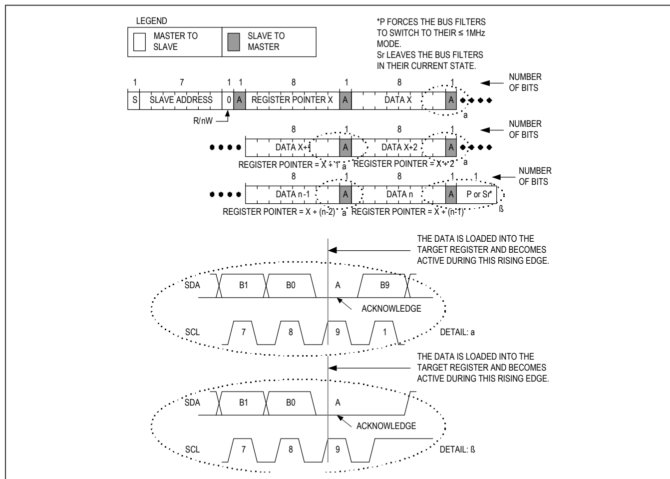
Figure 14. Writing to Sequential Registers X to N
