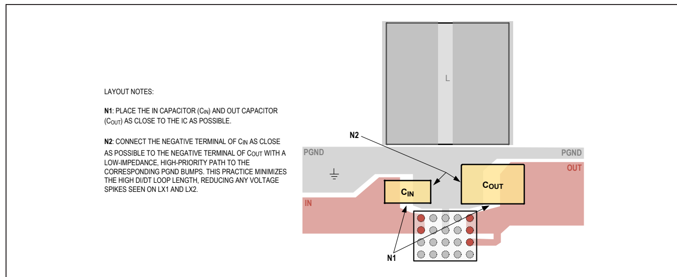
Figure 7. Recommended Capacitor Placement
