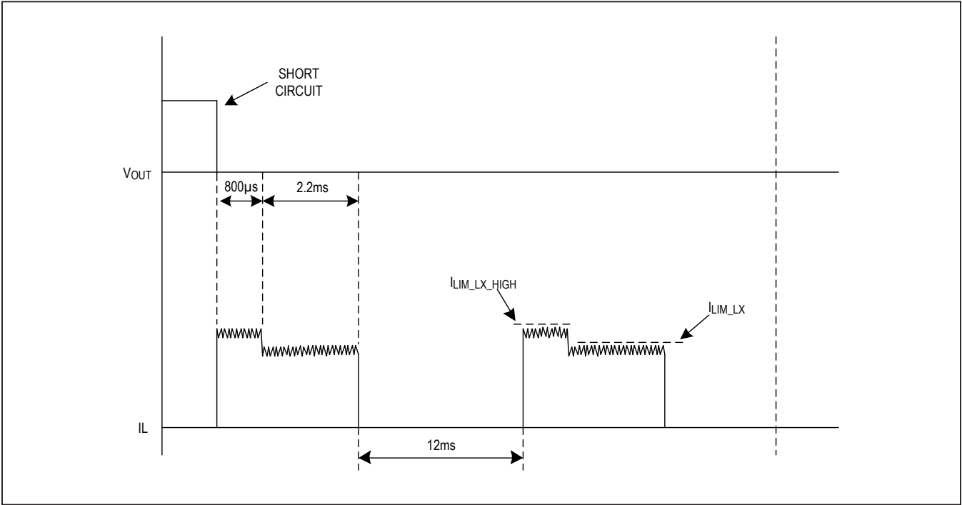
Figure 5. Short-Circuit Waveform
