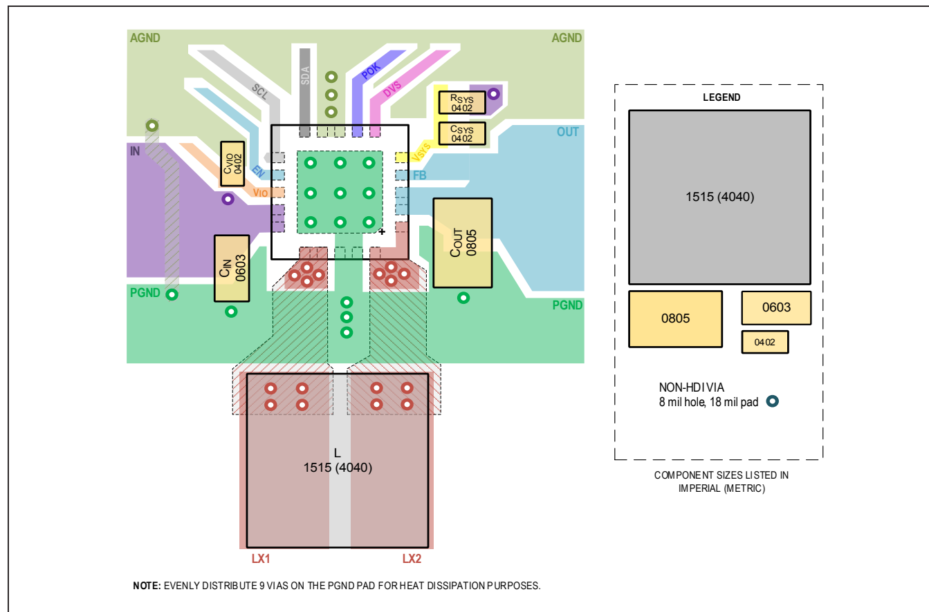
Figure 8. PCB Layout Example (TQFN)
