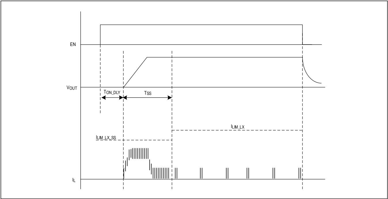
Figure 4. Startup Waveform
