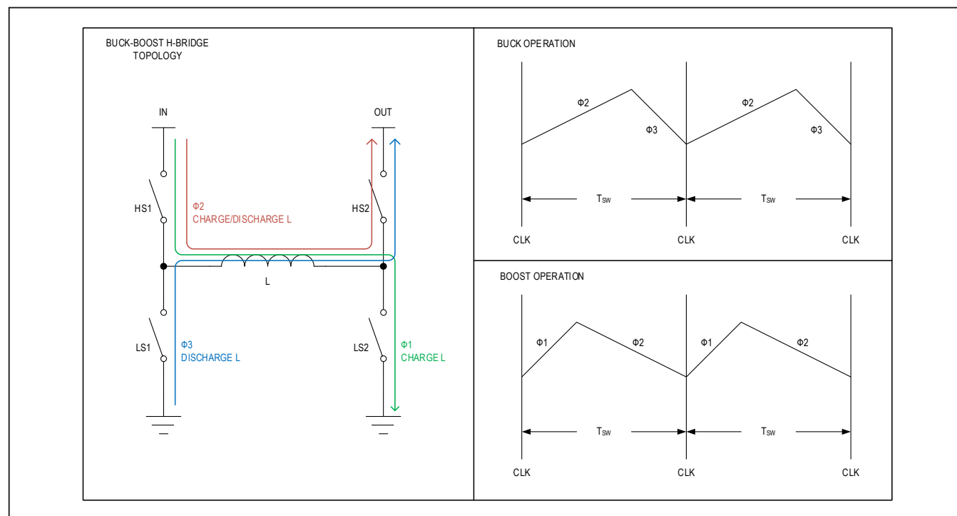
Figure 1. Buck-Boost H-Bridge Topology
