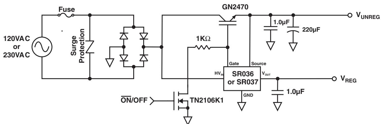
Figure 2: Example Circuit with Enable Control
