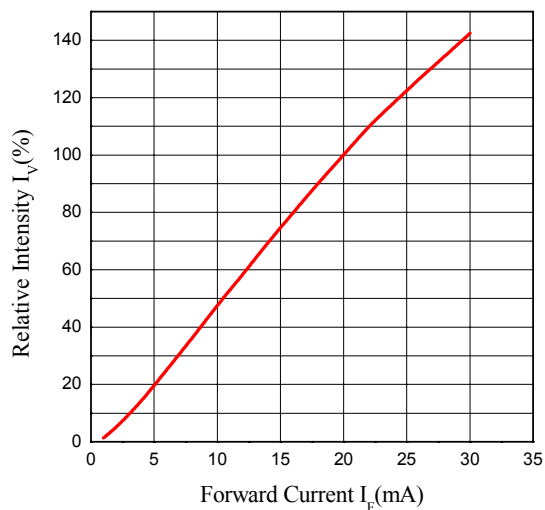
Relative Intensity I_v (%) vs Forward Current
