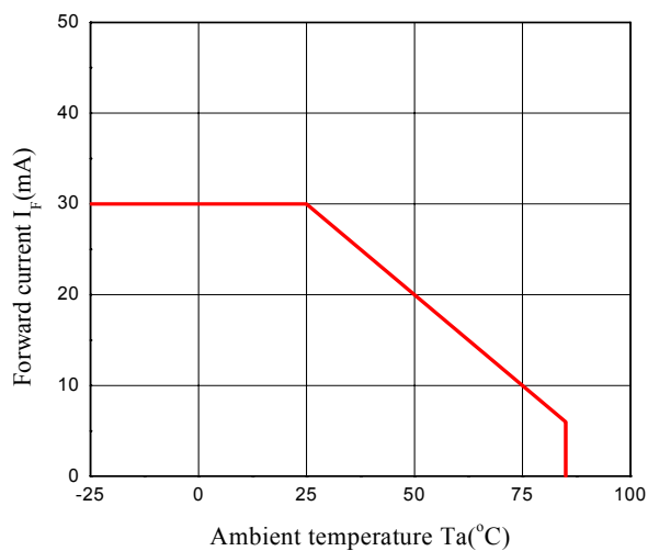
Forward Current vs Derating Curve
