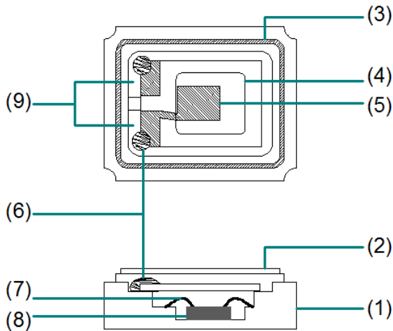
Reference drawing
