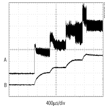
STARTUP WAVEFORMS
