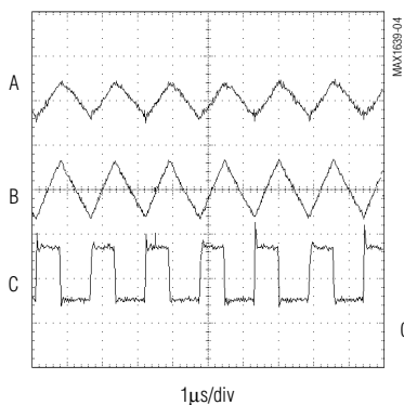
SWITCHING WAVEFORMS
