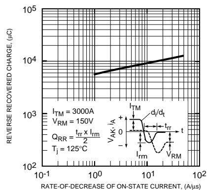
REVERSE RECOVERED CHARGE VS. RATE-OF-DECREASE OF ON-STATE CURRENT (TYPICAL)
