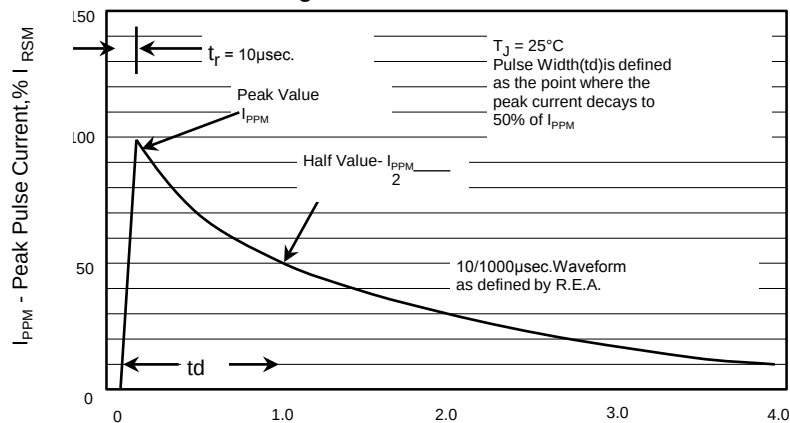
Fig.3 - Pulse Waveform
