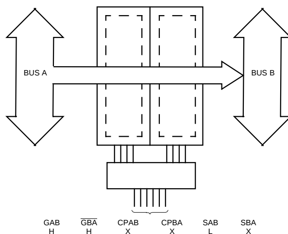
Real-Time Transfer Bus A to Bus B
