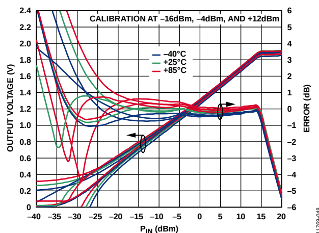
Figure 48. 2.14 GHz V_{RMS} and Log Conformance Error for Multiple Devices at +25^{\circ}\text{C} , -40^{\circ}\text{C} , and +85^{\circ}\text{C}
