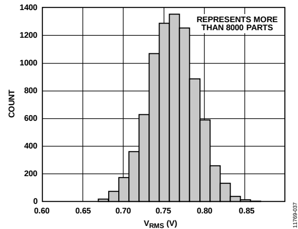
Figure 32. Distribution of V_{RMS} , P_{IN} = -16 dBm, 900 MHz
