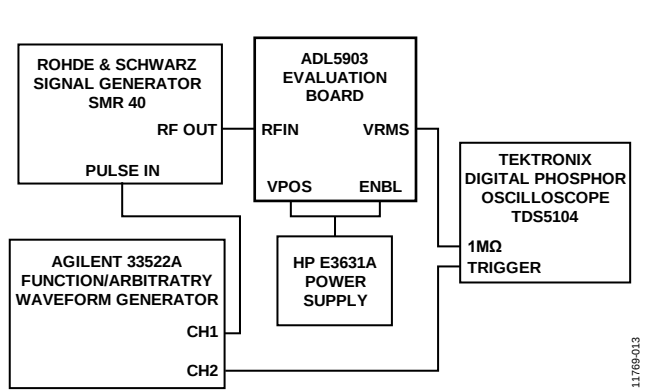
Figure 36. Hardware Configuration for Output Response to RF Burst Input Measurements
