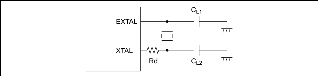
Figure 19.2 Connection of Crystal Resonator (Example)
