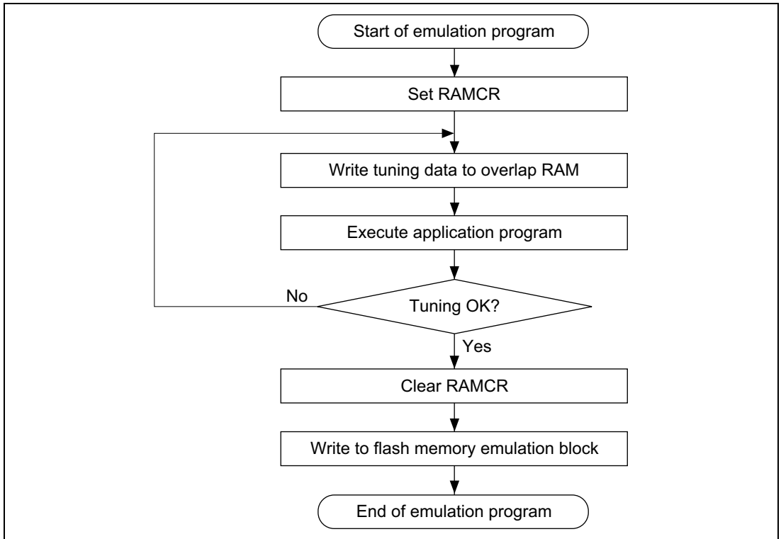
Figure 18.13 Flowchart of Flash Memory Emulation in RAM
