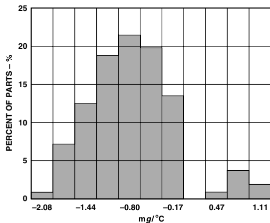
TPC 19. X-Axis Zero g Drift Due to Temperature Distribution, -40^{\circ}\text{C} to +85^{\circ}\text{C}
