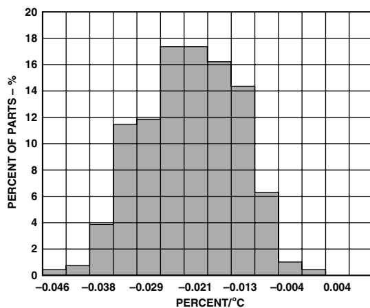
TPC 23. Y-Axis Sensitivity Drift at Y_{FILT} Due to Temperature Distribution, -40^{\circ}\text{C} to +85^{\circ}\text{C}
