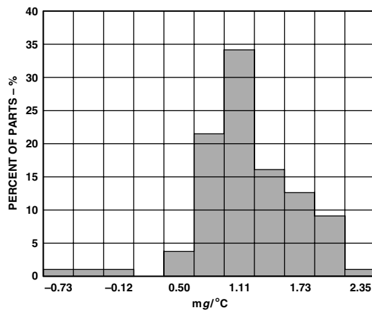
TPC 22. Y-Axis Zero g Drift Due to Temperature Distribution, -40^{\circ}\text{C} to +85^{\circ}\text{C}
