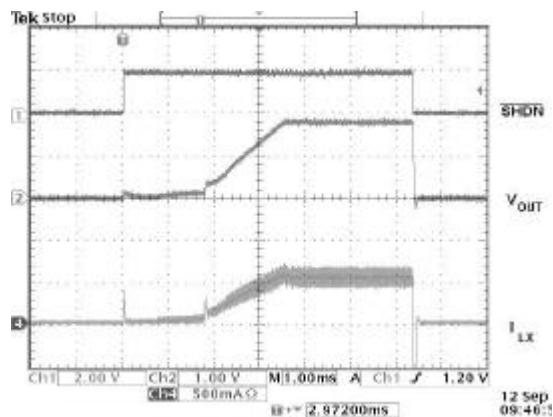
Fig. 16 Start-up from Shutdown, R_{LOAD}=3\Omega
