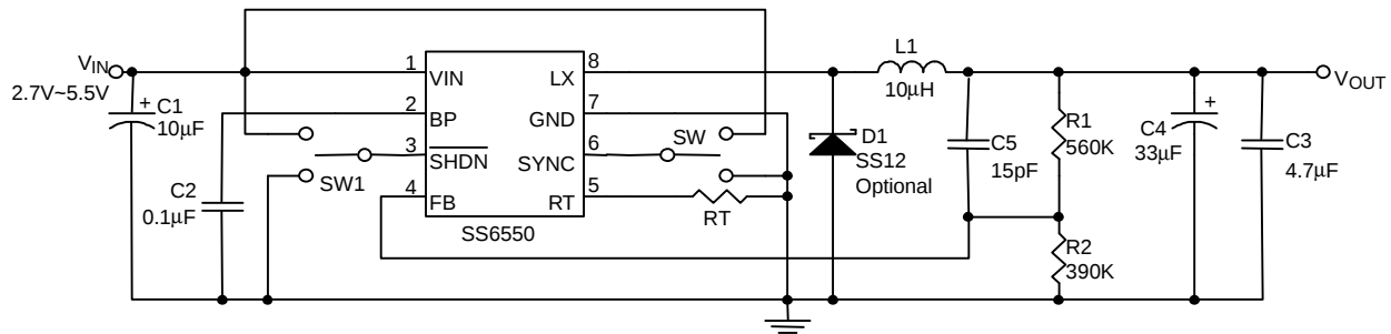
Fig. 22 SS6550 Application Circuit
