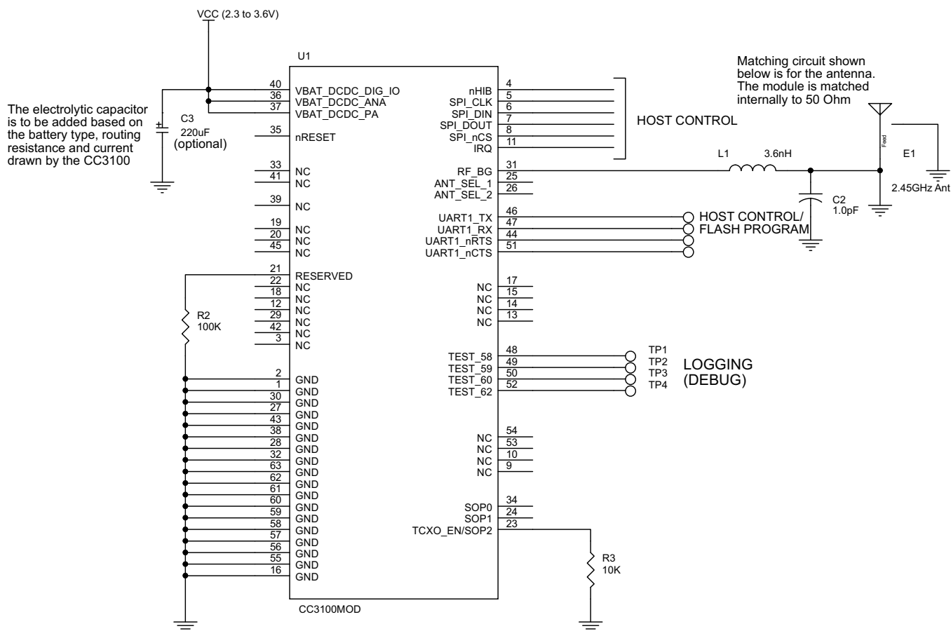
Figure 6-1. CC3100MOD Module Reference Schematic
