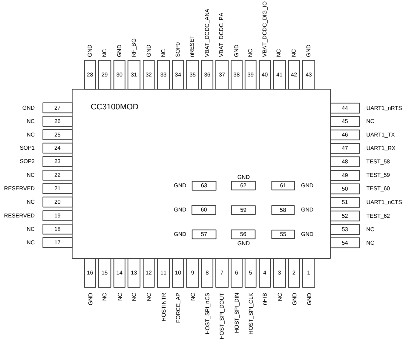
Figure 3-1. CC3100MOD Pin Diagram (Bottom View)
