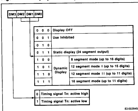
Figure 16. Display Mode Register Format
