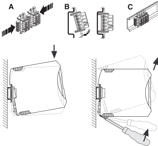
Figure 4 Mounting and removal
