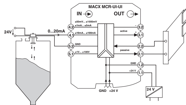
Figure 5 Example, level measurement
