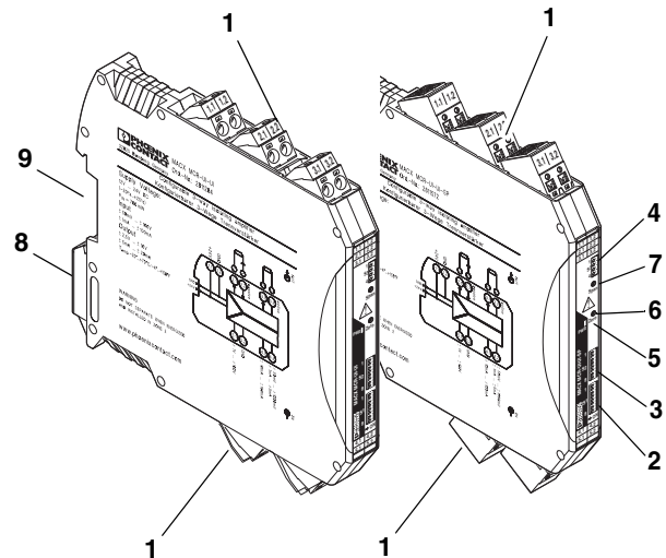
Figure 2 MACX MCR-UI-UI(-SP)(-NC) structure
