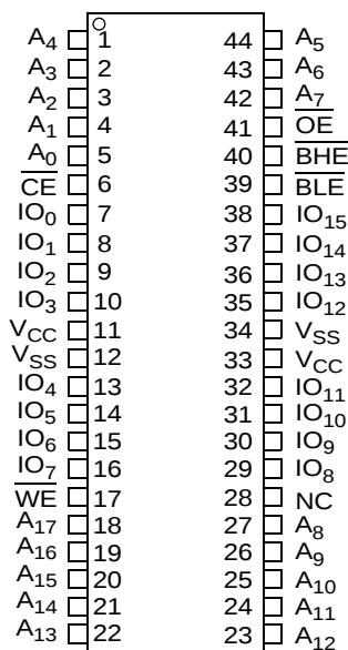
Figure 3. 44-Pin TSOP II [3]
