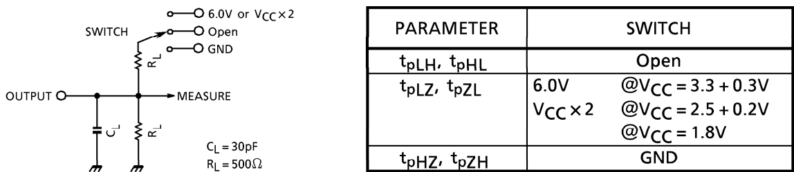
Fig.1 Test Circuit
