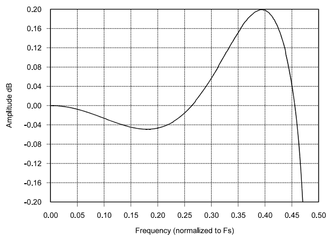
Figure 17. Double-Speed Passband Ripple
